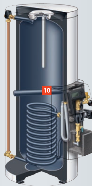
Vitocell 100-W (type CVSA)
